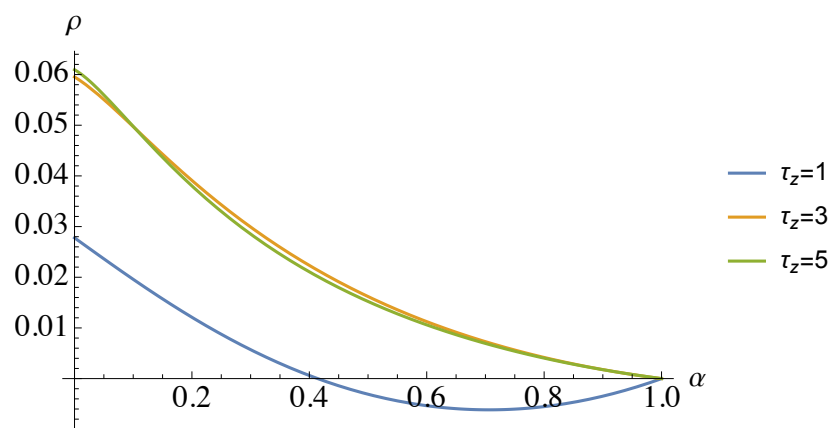
Figure 1: A plot of \rho vs. \alpha Other parameters are \tau_V = \tau_\varepsilon = \gamma = 1 .
